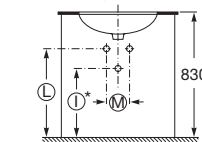
Semi-recessed
