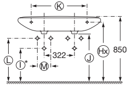
Wall-hung/Double wall-hung
