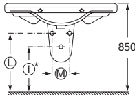
Semi-pedestal
