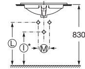
Countertop basins
