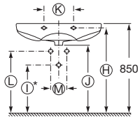
Wall-hung/Double wall-hung
