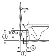
Dual outlet
