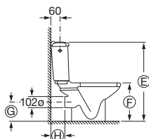
Horizontal outlet
